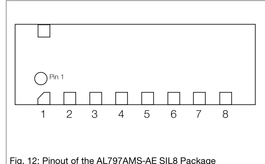
Fig. 12: Pinout of the AL797AMS-AE SIL8 Package
